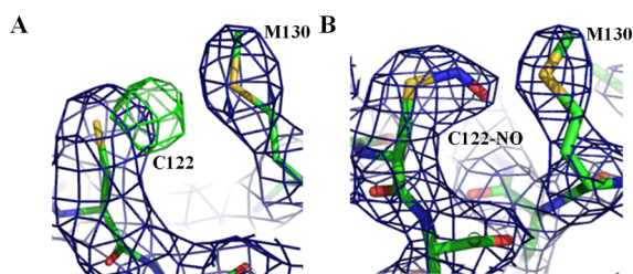
Figure 6. Electron density maps showing S-nitrosylation of C122 of Ns H-NOX. 2F_o - F_c electron density map in blue contoured at 1\sigma and F_o - F_c electron density map in green contoured at 3\sigma . (A) Green density near C122 showing S-nitrosylation difference density of C122 prior to modeling residue as an S-nitrosylated cysteine (in molecule A). (B) 2F_o - F_c electron density map in blue contoured at 1\sigma of S-nitrosylated C122.
