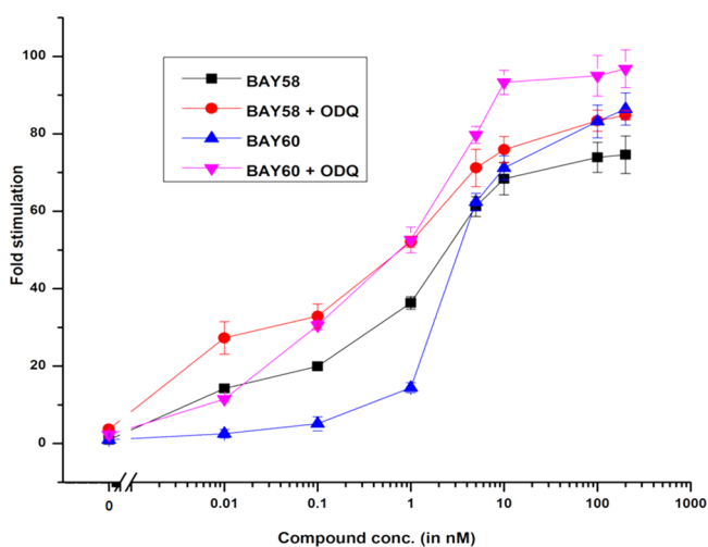
Figure 3. Activation effects of bovine sGC by BAY 58-2667 and BAY 60-2770 in the absence and presence of ODQ (10 \mu M).
