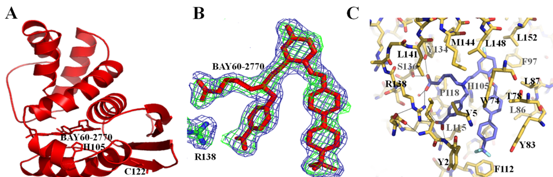
Figure 4. BAY 60-2770 interactions in Ns H-NOX. (A) Cartoon representation of BAY 60-2770 (in sticks) complexed to C139A Ns H-NOX (molecule A); H105 and C122 are shown in sticks. (B) 2F_o - F_c electron density contoured at 1\sigma in blue and omit F_o - F_c density contoured 2.5\sigma in green color for BAY 60-2770 within heme cavity. (C) Interactions of BAY60-2770 with nearby H-NOX residues, hydrogen bonds are shown as dashed lines.
