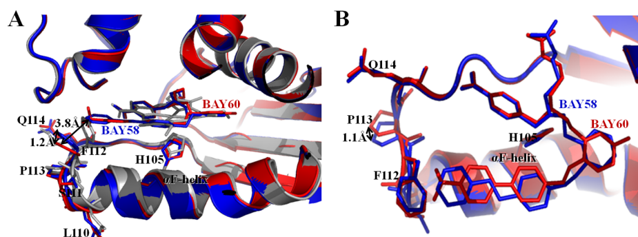
Figure 5. Comparison between BAY 58-2667 and BAY 60-2770 bound Ns H-NOX structures. BAY 58-2667 bound Ns H-NOX structure in blue color and BAY 60-2770 bound C139A Ns H-NOX structure in red color. (A) Side view of cartoon superposition of BAY 58 bound and BAY 60 bound H-NOX structures showing no structural change in \alpha F-helix while its C-terminus loop region 110–114 is altered; side chains of loop region residues are shown in sticks and BAY 58 and BAY 60 drug molecules are shown in blue and red stick models, respectively. As a reference, the superimposed heme-bound protein structure of H-NOX is shown in gray. (B) Top view of panel (A), distances between side chain positions are shown with double-head arrows. BAY 58-2667 and BAY 60-2770, H105 of \alpha F-helix and loop residues — L110, S111, F112, P113, Q114 are shown in sticks.
